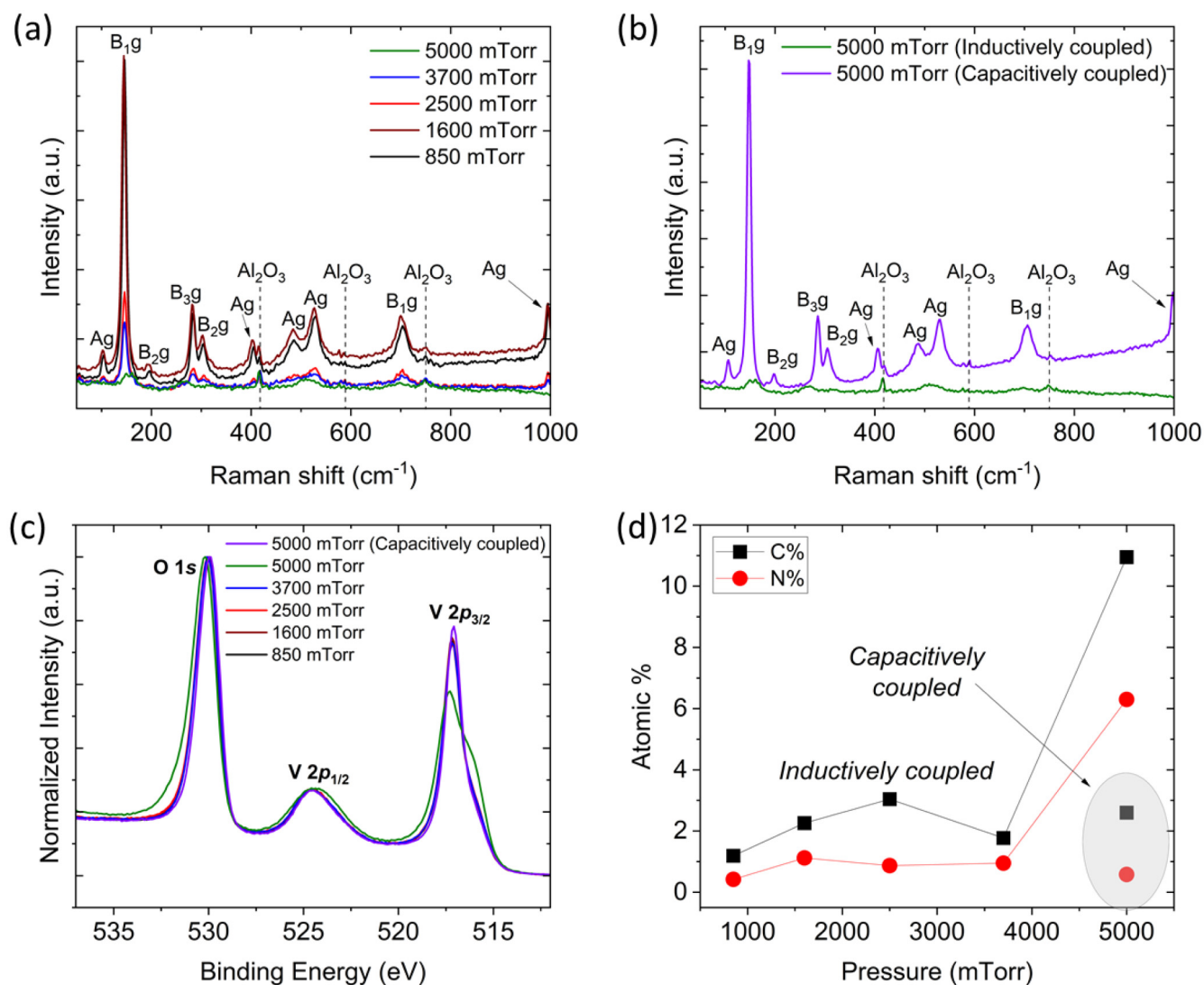
FIG. 7. (a) Raman spectra of VO x as a function of pressure during the plasma step for plasmas operated in an inductively coupled mode. (b) A comparison of Raman spectra of VO x deposited with inductively and capacitively coupled plasmas at 5000 mTorr. XPS of (c) the O 1s and V 2p core levels as a function of pressure (plasmas operated in an inductively coupled mode unless otherwise noted) and (d) C and N contamination as a function of pressure during the plasma step.
