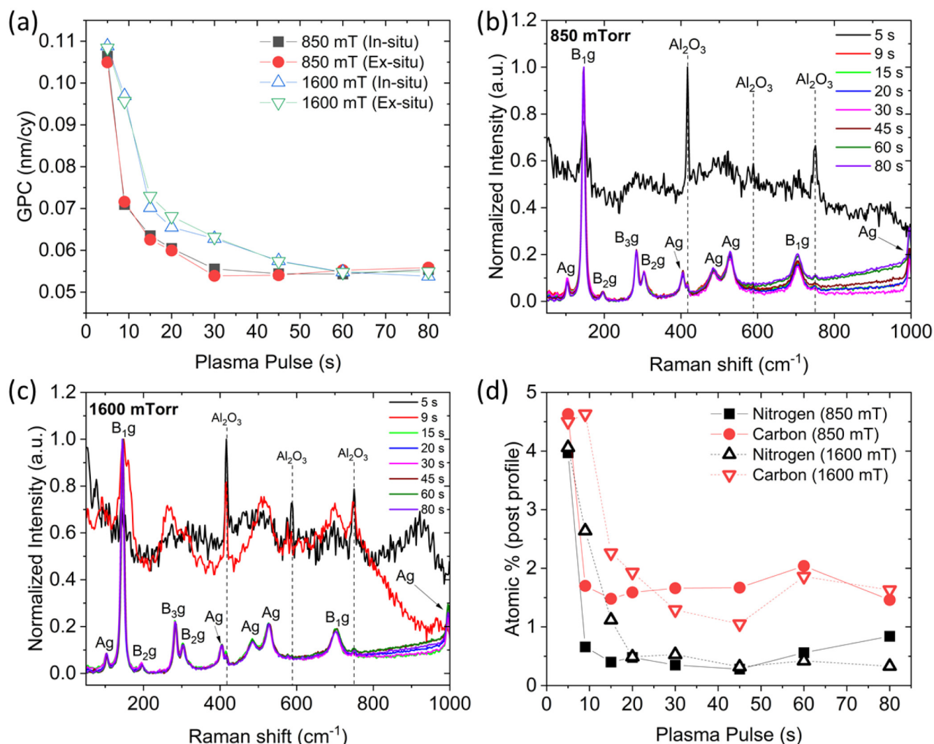
FIG. 2. (a) GPC of \text{VO}_x as a function of plasma pulse duration at 850 and 1600 mTorr. Normalized Raman spectra of \text{VO}_x deposited as a function of plasma pulse duration at 850 (b) and 1600 mTorr (c). (d) XPS-derived N and C atomic % as a function of plasma pulse duration at 850 and 1600 mTorr.
