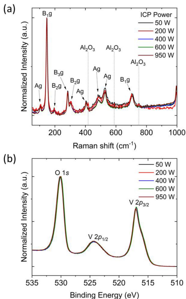
FIG. 3. (a) Normalized Raman spectra and (b) XPS V 2p and O 1s peaks of VO x deposited at 850 mTorr with varying plasma power.
